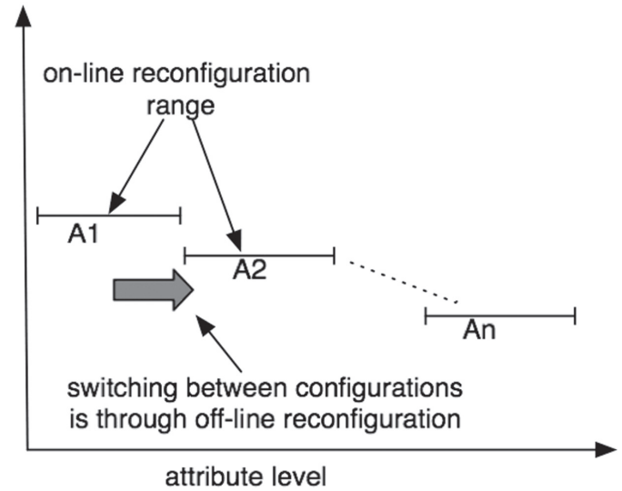
Fig. 15 On-line and Off-line reconfiguration.
