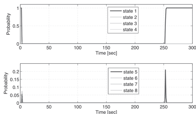
Fig. 10 Evolution of state probabilities – a.
