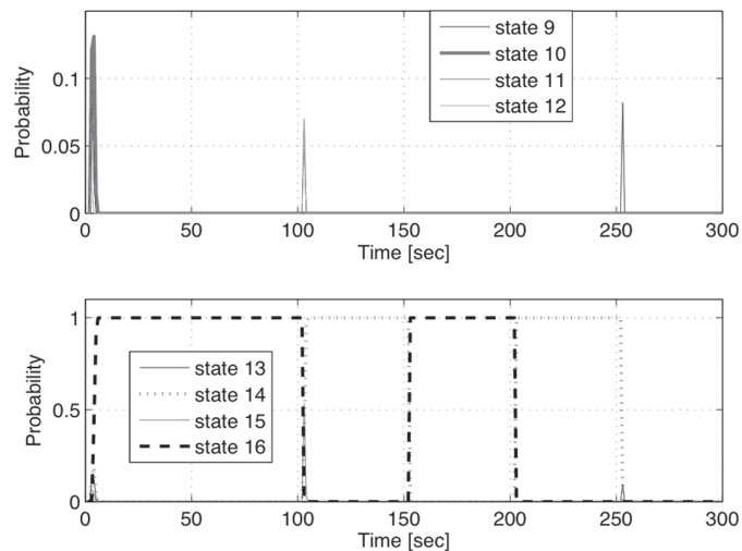
Fig. 9 Evolution of state probabilities – b.
